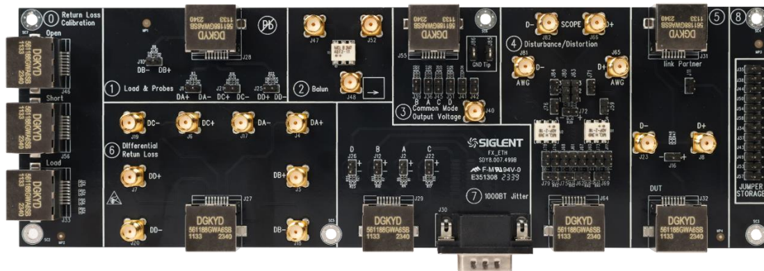
Figure 1 Ethernet Electrical Compliance Test Fixture Board
