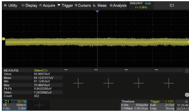
Low noise floor: Only 70 \mu Vrms at 200 MHz bandwidth
