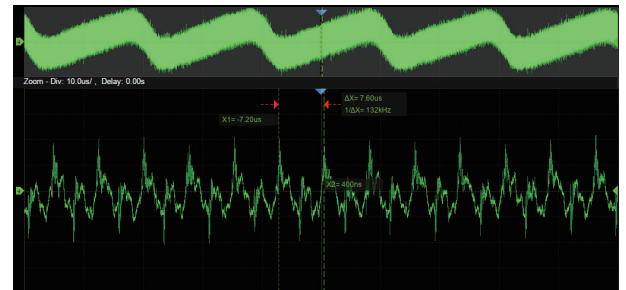
Using hardware-based Zoom technique and record length of up to 200 Mpts, users can select a slower timebase without compromising the sample rate, and then quickly zoom in to focus on the area of interest
