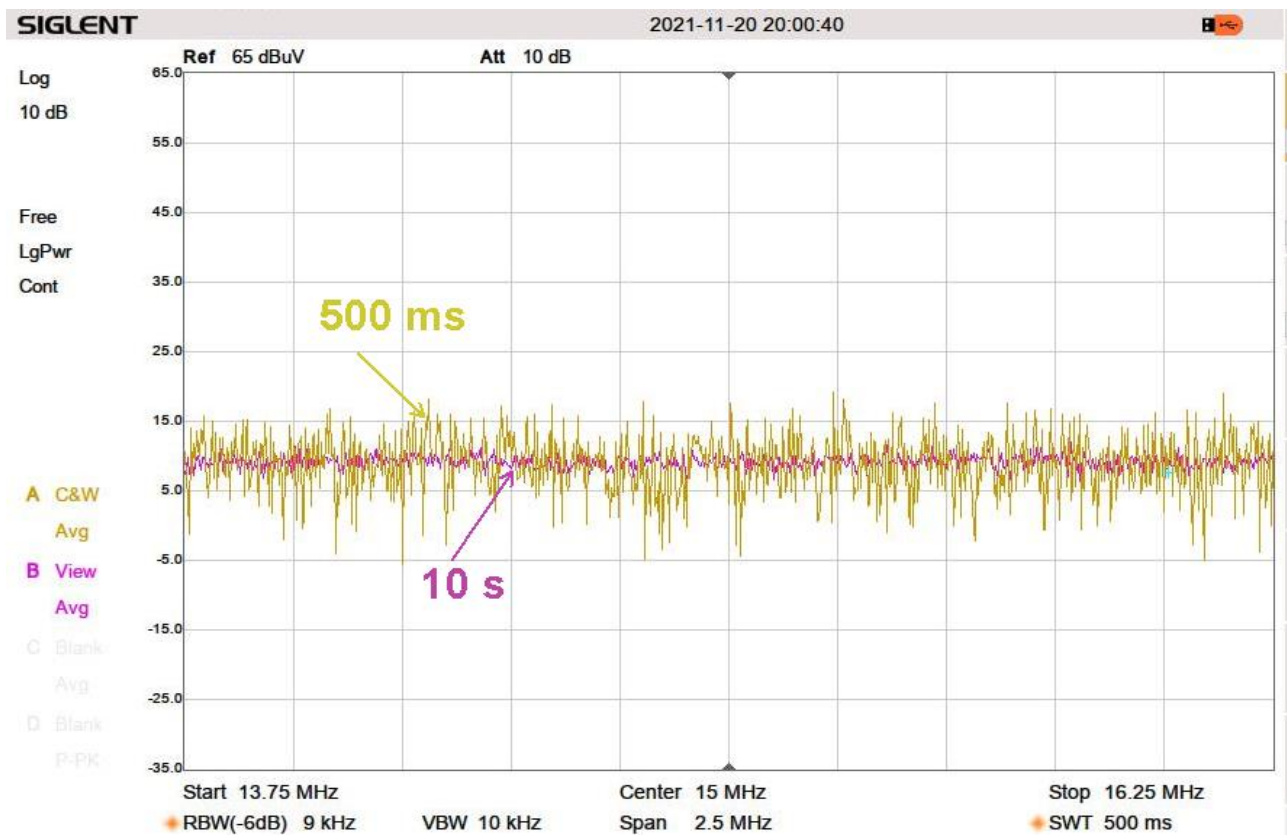
Base noise with 500 ms sweep time versus 10 s sweep time
