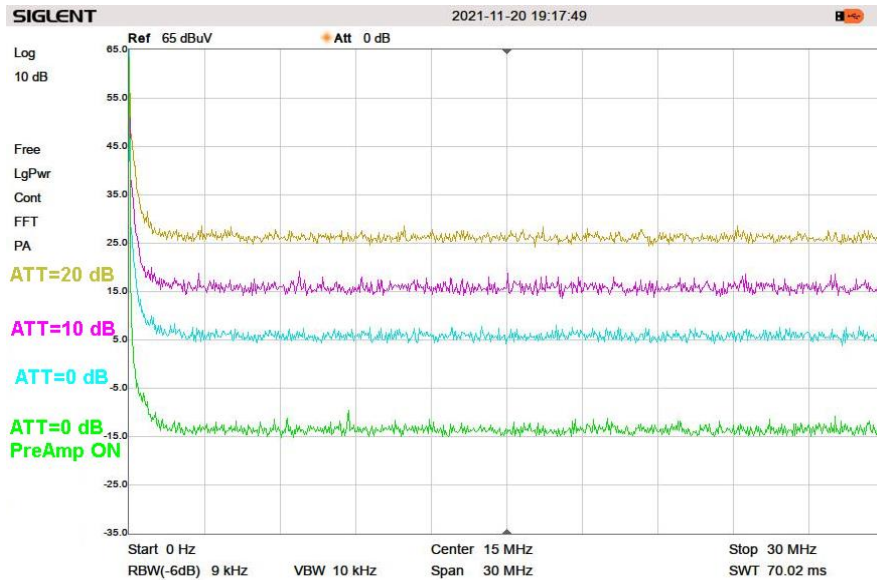
Spectrum analyzer base noise versus internal attenuator / pre-amplifier settings. RF input terminated with 50 Ohm
